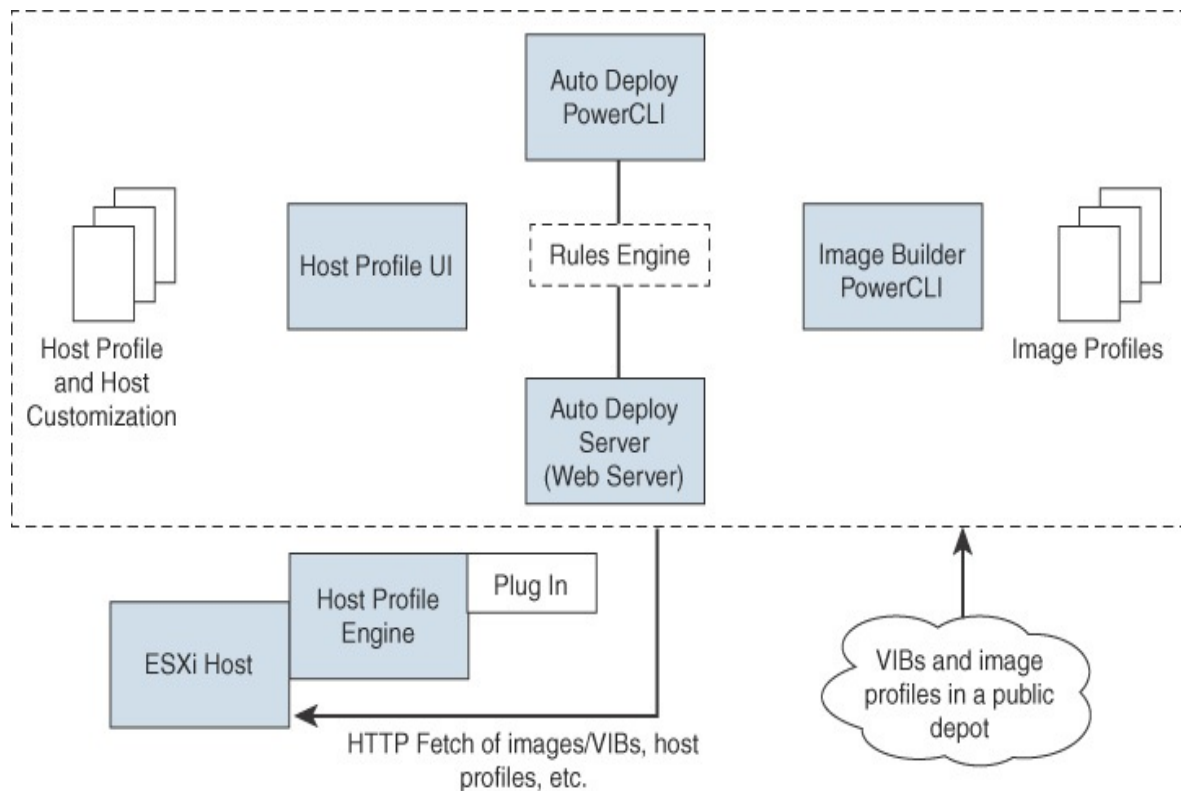
FIGURE 8-2 Auto Deploy Architecture
