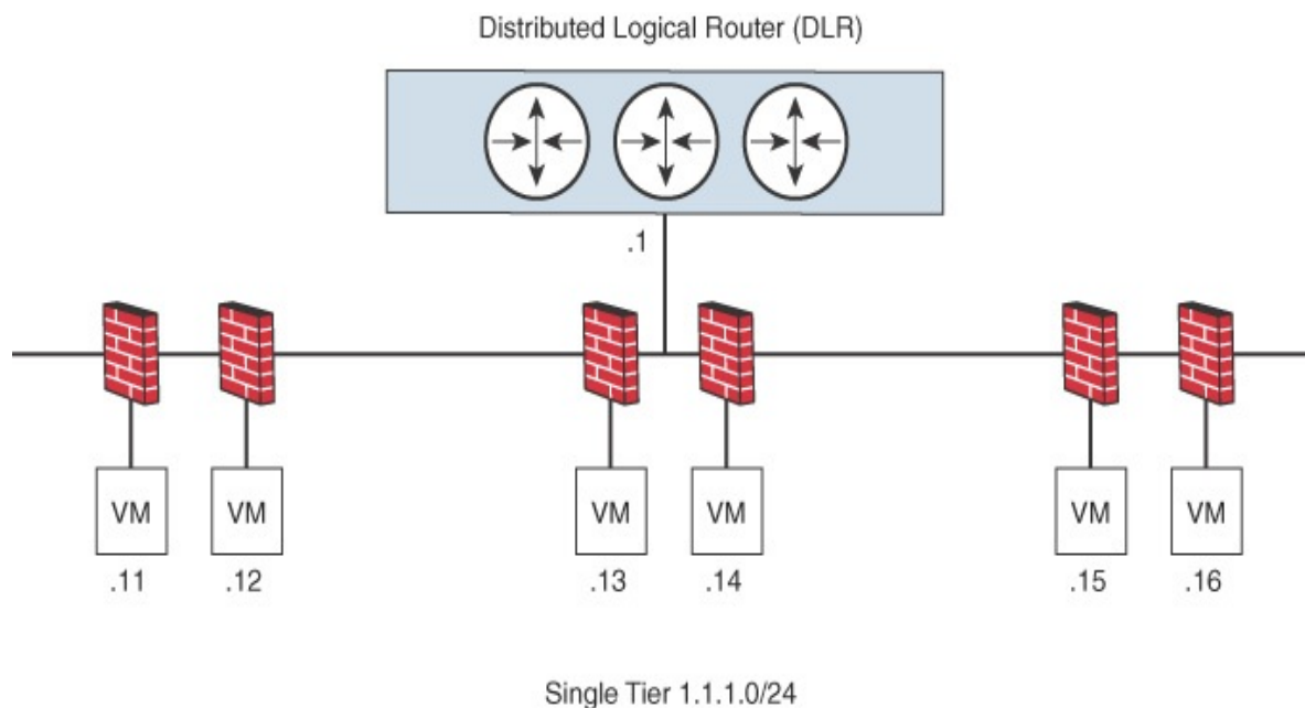
FIGURE 7-7 Example with a Single Layer 2 Segment
