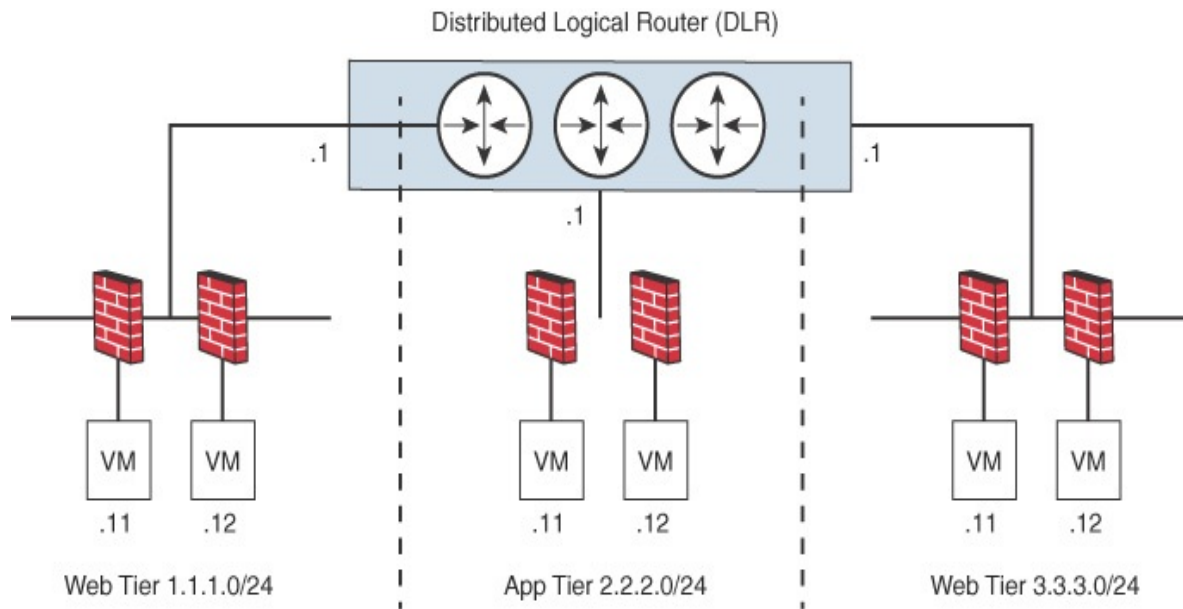
FIGURE 7-6 Example with Multiple Layer 2 Segments
