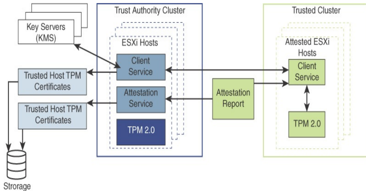
FIGURE 7-5 vSphere Trusted Authority Architecture
