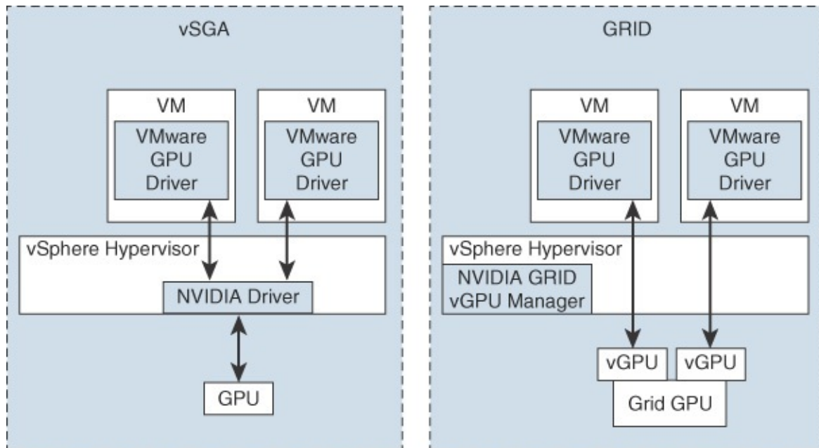
FIGURE 14-1 Comparison of the vSGA and GRID Models
