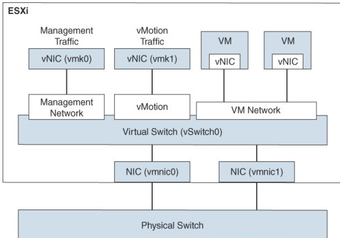
FIGURE 3-1 A Sample Virtual Switch
