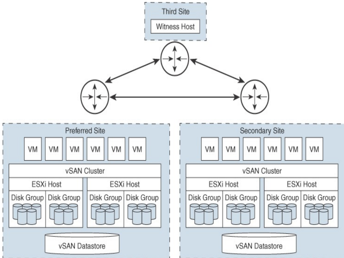
FIGURE 2-5 A Stretched vSAN Cluster
