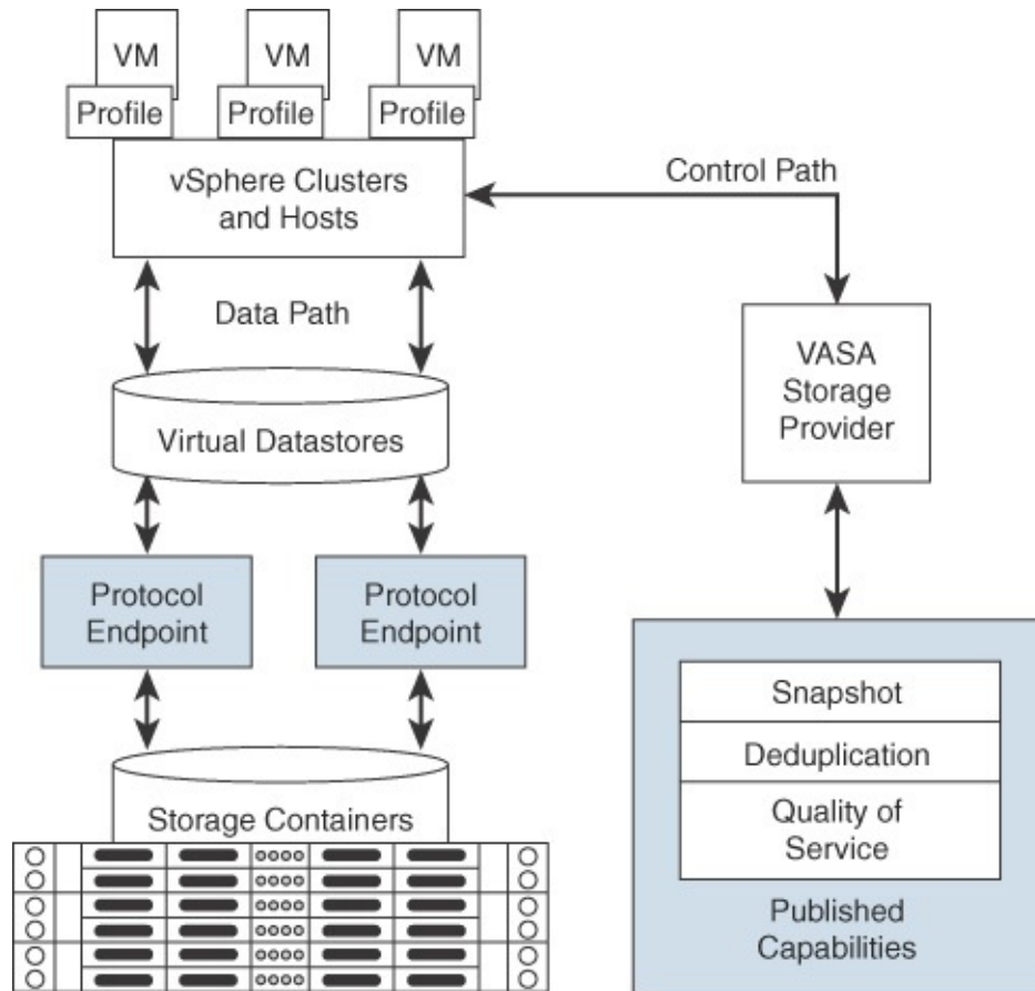
FIGURE 2-7 vVols Architecture
