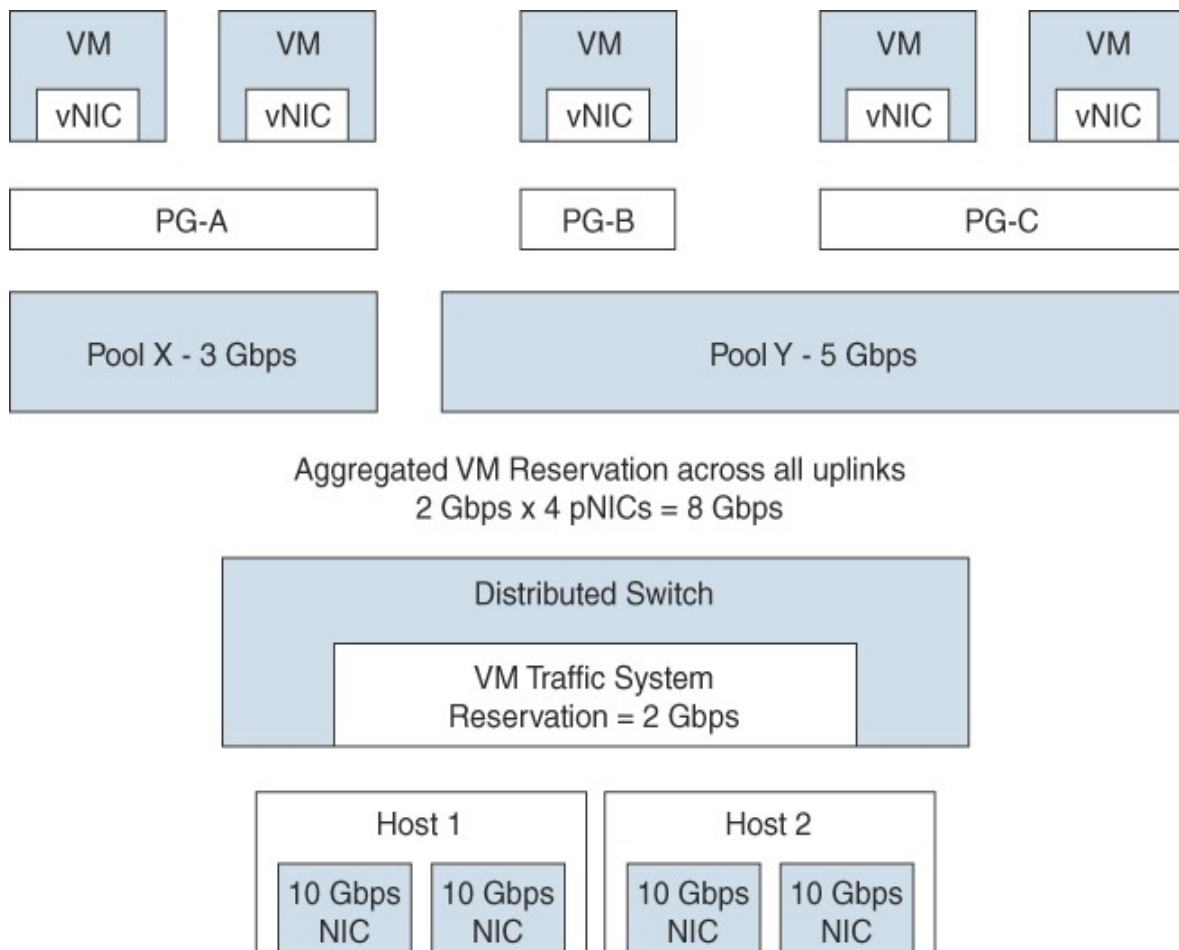
FIGURE 3-3 Network Resource Pools Example
