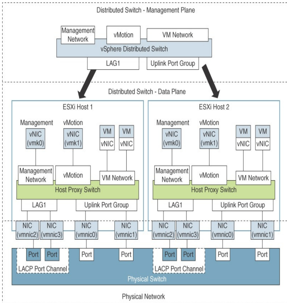
FIGURE 3-4 LACP Configuration with a vDS
