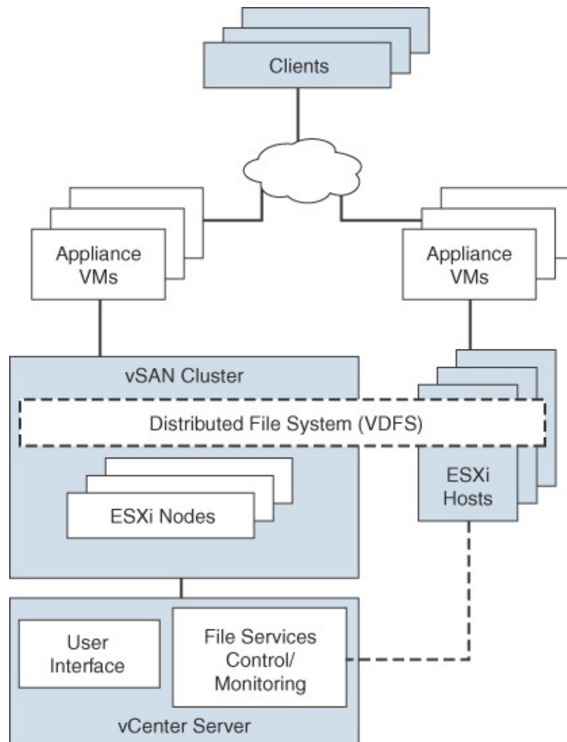
FIGURE 2-6 vSAN File Services Architecture
