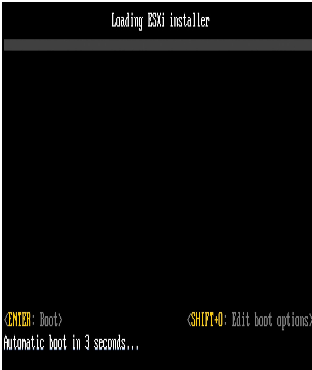
FIGURE 8-1 ESXi Installer
