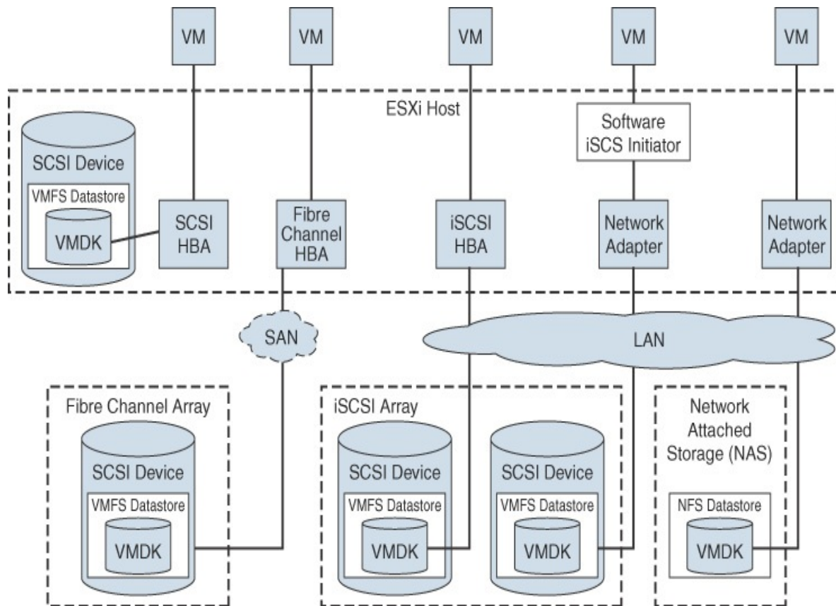
FIGURE 2-1 Virtual Machine Storage
