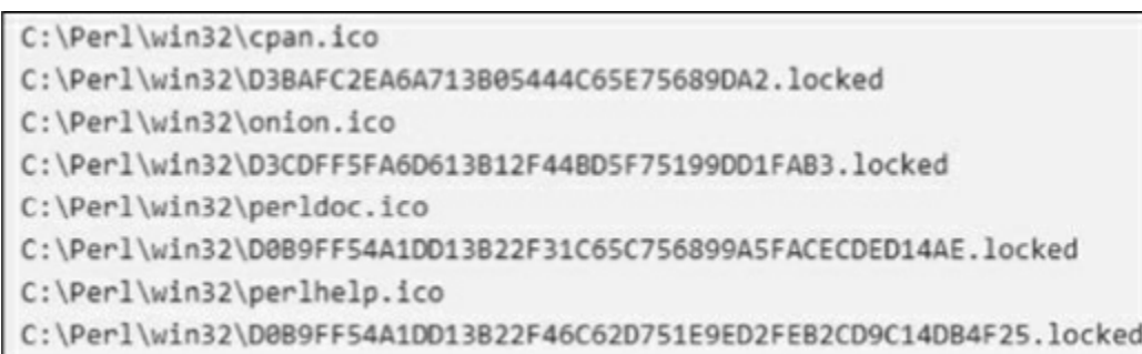
Figure 3-6: File paths in the Files tab of the Summary pane, suggesting that our sample is ransomware
