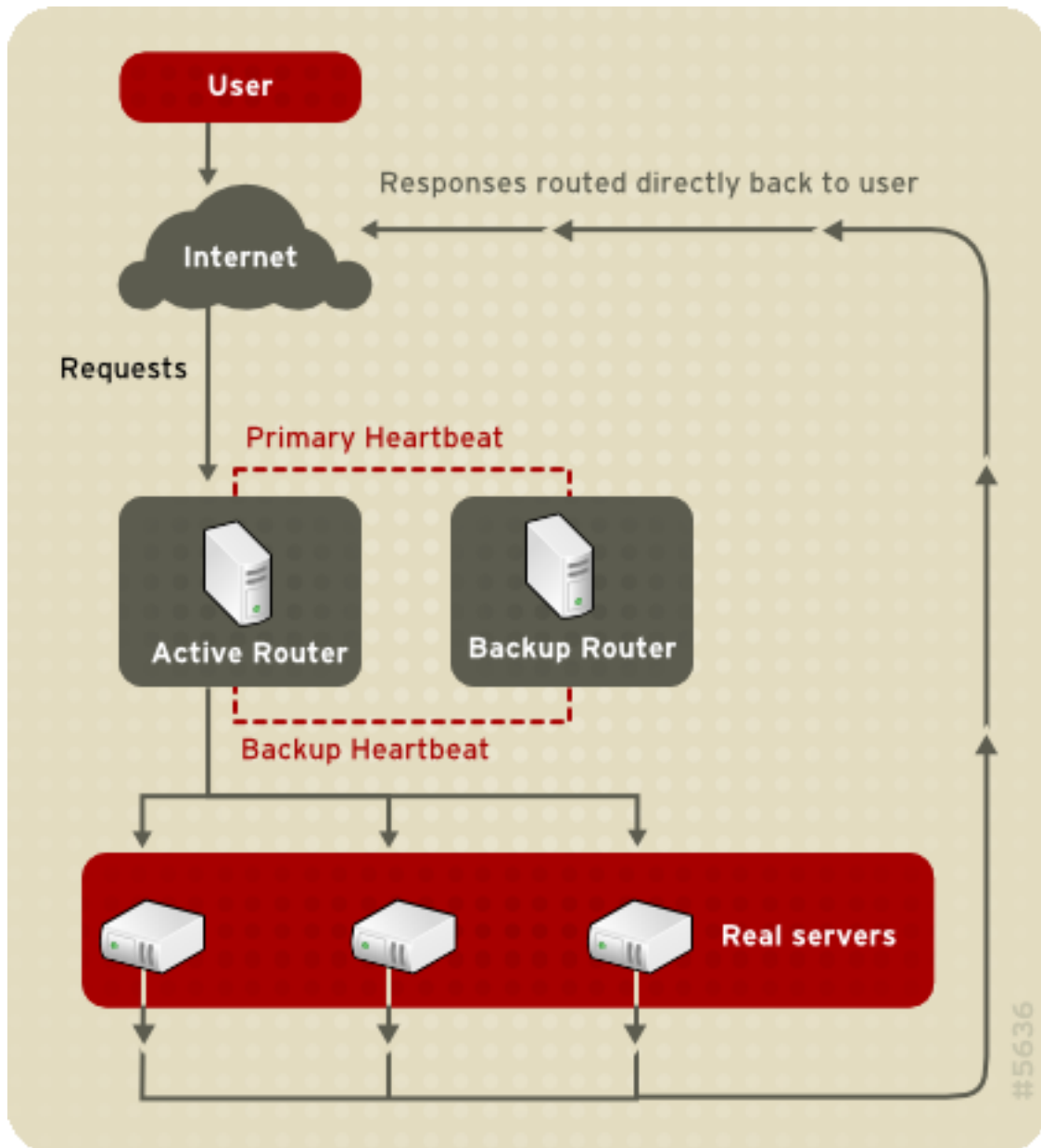
Figure 2.4. An LVS Cluster Implemented with Direct Routing
