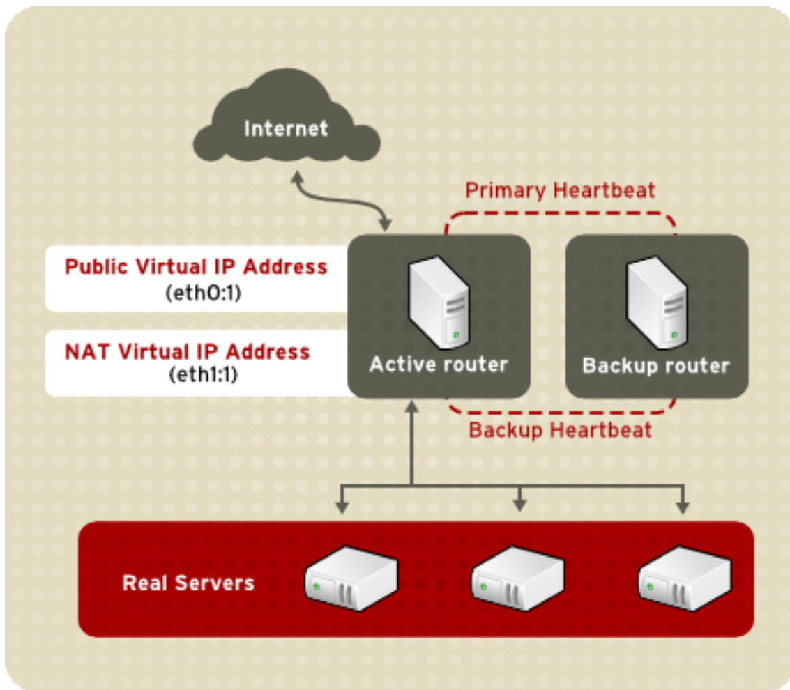
Figure 2.3. An LVS Cluster Implemented with NAT Routing
